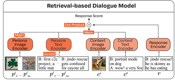
Figure 4: The architecture of retrieval-based model for the next response prediction task.
